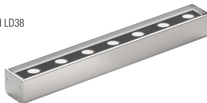
LD38C Integrated linear anti-glare cowl, supplied with special end caps to further reduce glare from the sides
